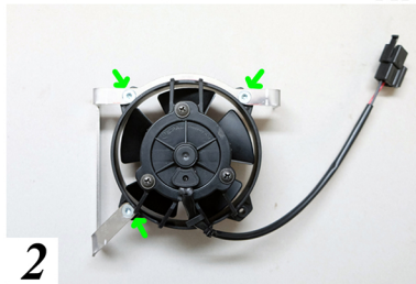
Fig.2 Montare staffa sulla ventola/ Fig.2 Mount bracket on the fan
