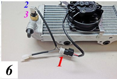
Fig. 6-7 collegare ventola al bulbo tramite connettori (1-2-3)/ Fig. 6-7 connect fan to bulb via connectors (1-2-3-)
